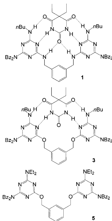
Scheme 1. Illustration of the target bis(triazine) receptor–barbital interactions, appropriate substitution of the triazine allows modulation of the number of hydrogen-bonding acceptor and donor sites allowing a degree of control over the strength of the host–guest interaction.
