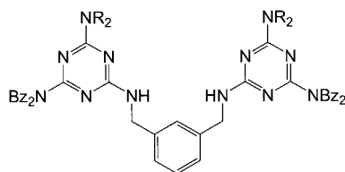
Scheme 4. Targeted-amine-substituted bis(triazine) receptor molecules, \text{R} = \text{Bz} , \text{Bu} , \text{Et} .
