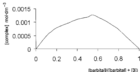
Figure 1. Job plot of [Complex] vs. [Host]/([Host] + [Guest]) for barbitaral and 3 .
