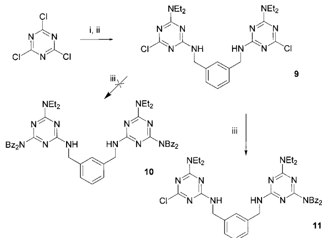
Scheme 5. i. 1,3-Xylylenediamine, DIPEA, THF, 0^\circ\text{C} ; ii. diethylamine, DIPEA, THF, room temp.; iii. (\text{PhCH}_2)_2\text{NH} , DIPEA, refluxing THF.
