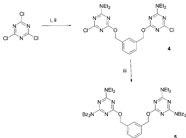
Scheme 3. i. 1,3-Benzenedimethanol, 2,6-lutidine, room temp. \text{CH}_2\text{Cl}_2 ; ii. diethylamine, 2,6-lutidine, room temp. \text{CH}_2\text{Cl}_2 ; iii. (\text{PhCH}_2)_2\text{NH} , DIPEA, refluxing THF.
