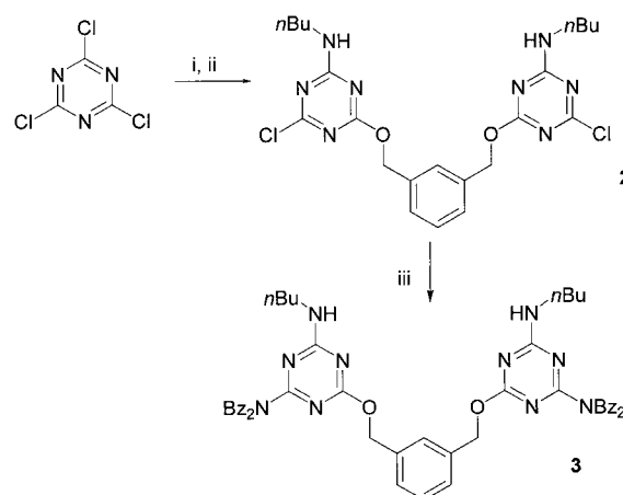
Scheme 2. i. 1,3-Benzenedimethanol, 2,6-lutidine, room temp. CH 2 Cl 2 ; ii. butylamine, 2,6-lutidine, room temp. CH 2 Cl 2 ; iii. (PhCH 2 ) 2 NH, refluxing THF.
